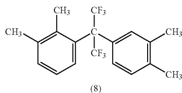
Scheme IV Alternative Synthesis of a-6FDA
